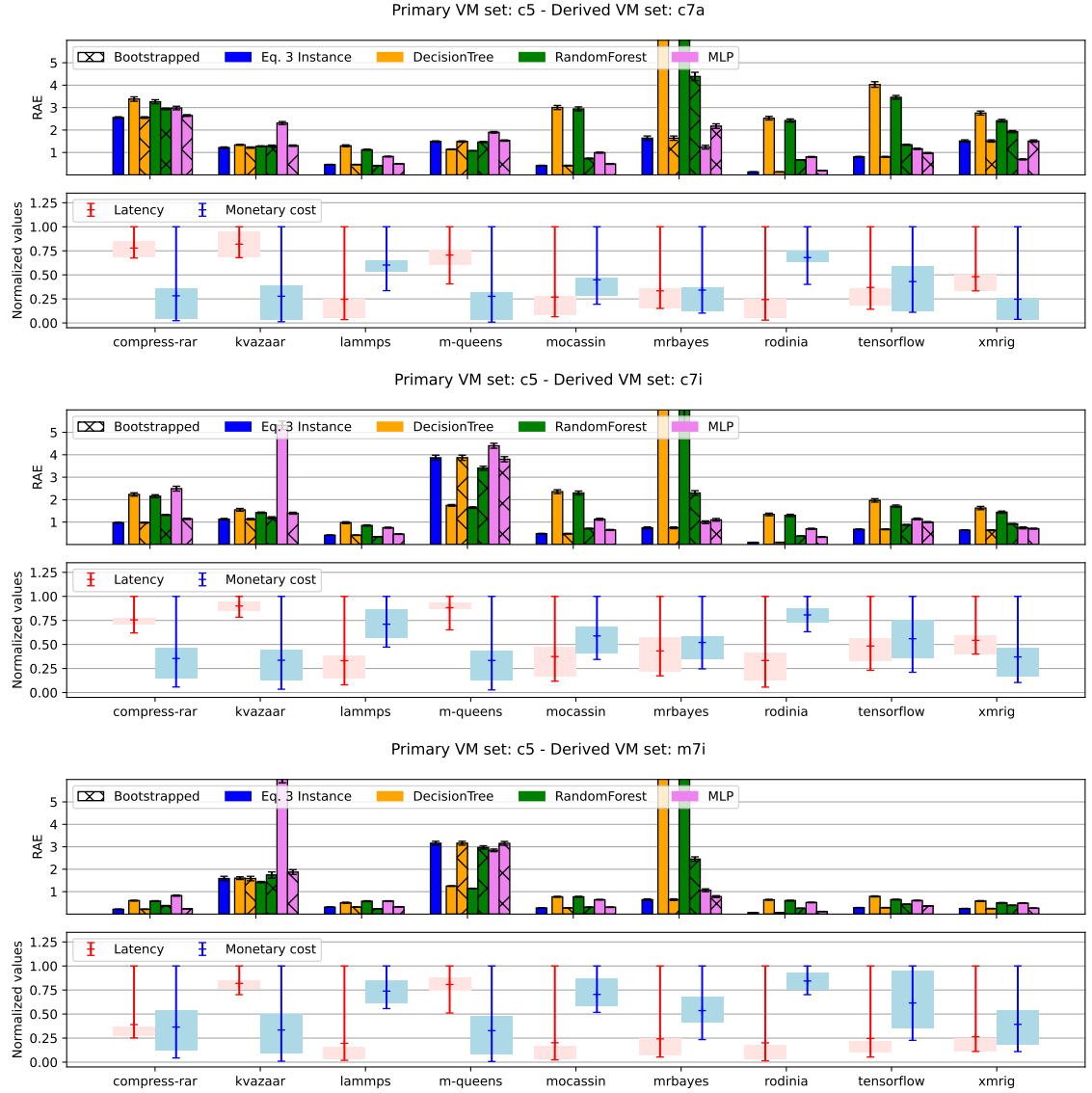
Fig. 5. Results for C7a, C7i and M7i families for all benchmark applications, using C5 family as a primary VM set, three samples ( k = 3 ) for the primary VM set and one sample for each.
